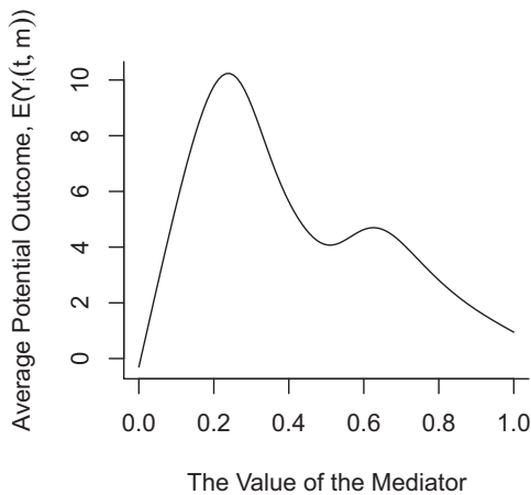
Figure E1. Nonlinear relationship used for a Monte Carlo study. The solid line represents the average potential outcome, \mathbb{E}(Y_i(t, m)) , as a function of the mediator while the treatment variable is held constant.
